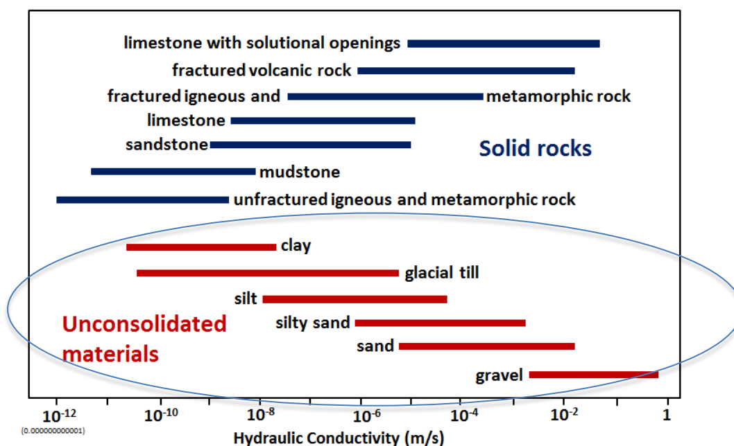
Figure 10: Variations in hydraulic conductivity (how quickly a fluid flows through the material in meters/second) of unconsolidated materials (circled) and rocks.
