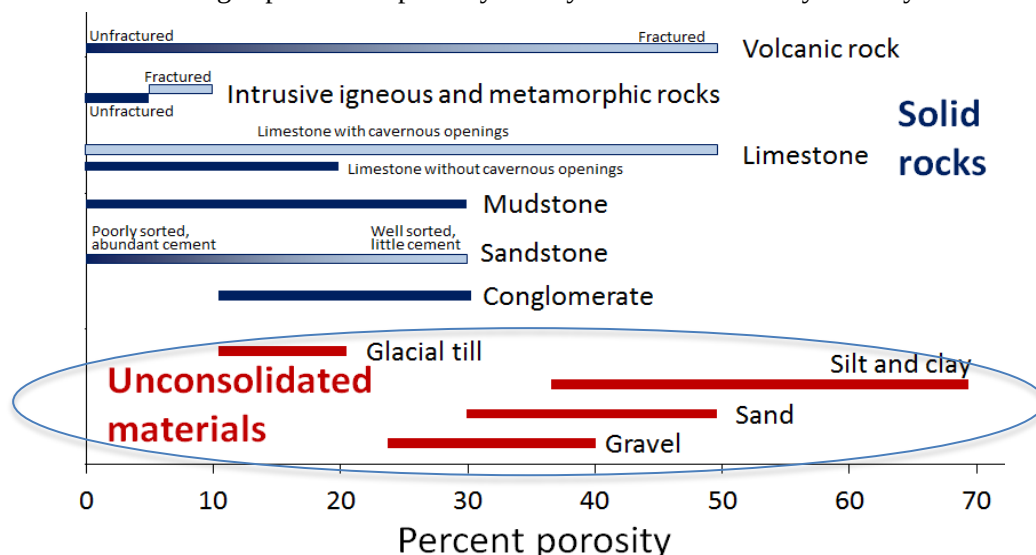
Figure 9: Variations in porosity of unconsolidated materials (circled red bars) and rocks (blue bars). Note: Porosity is the void-space portion of a rock as a percentage of the total volume of the rock.
