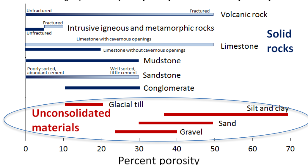
Figure 9: Variations in porosity of unconsolidated materials (circled red bars) and rocks (blue bars).
