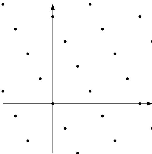
Figure 1: An example of a lattice.
