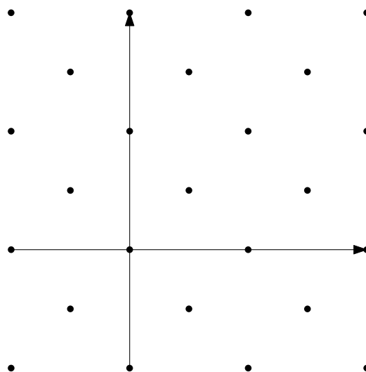
Figure 2: The lattice generated by \{(1, 1), (1, -1)\} .
